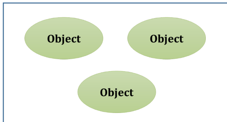
Figure 1.1.4: Heap
