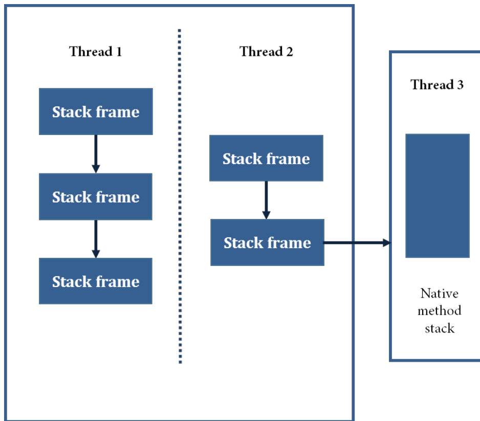
Figure 1.1.3: Stack Mechanism
